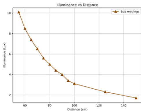
Even Measurement radiation for 50mm board.
