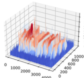
Even Measurement radiation for 75mm board.
