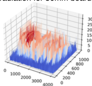
Even Measurement radiation for 50mm board.
